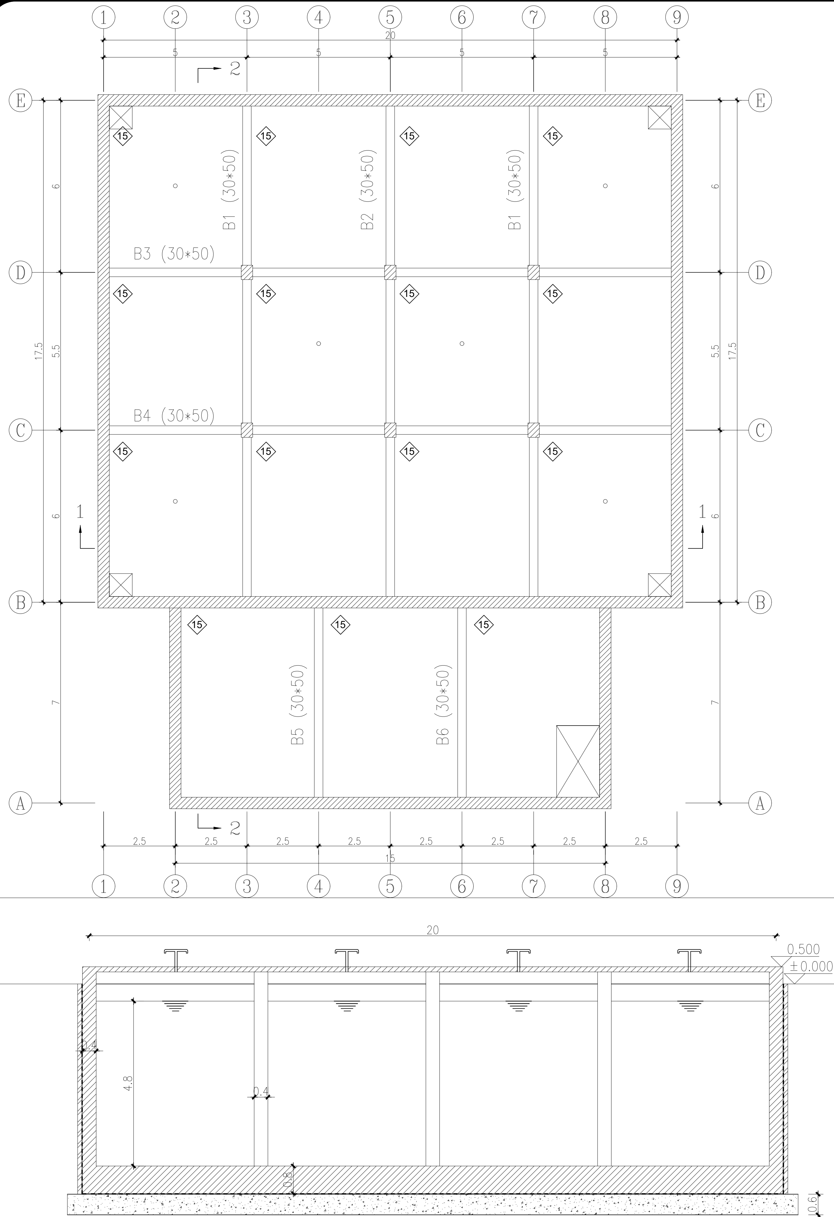
Section 1-1
